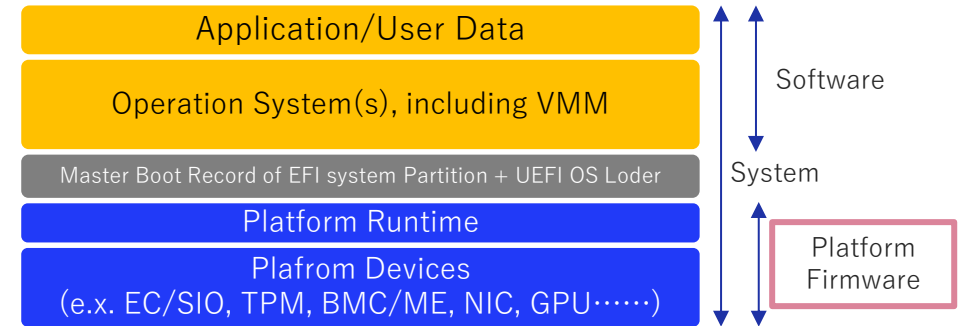
Fig.1 Hight-Level System Architecture
